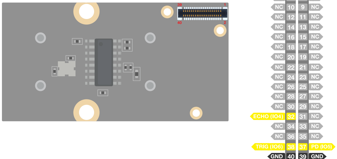
Figure 5: RAK12007 WisBlock Ultrasonic Sensor Module Pinout
