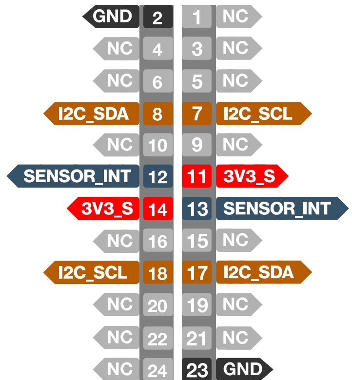
Figure 2: RAK12021 pinout
