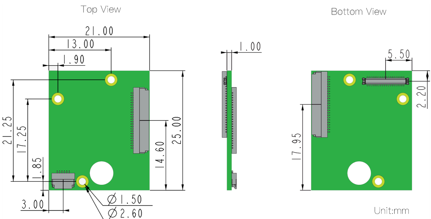
Figure 3: RAK14000 Module Mechanical Characteristics
