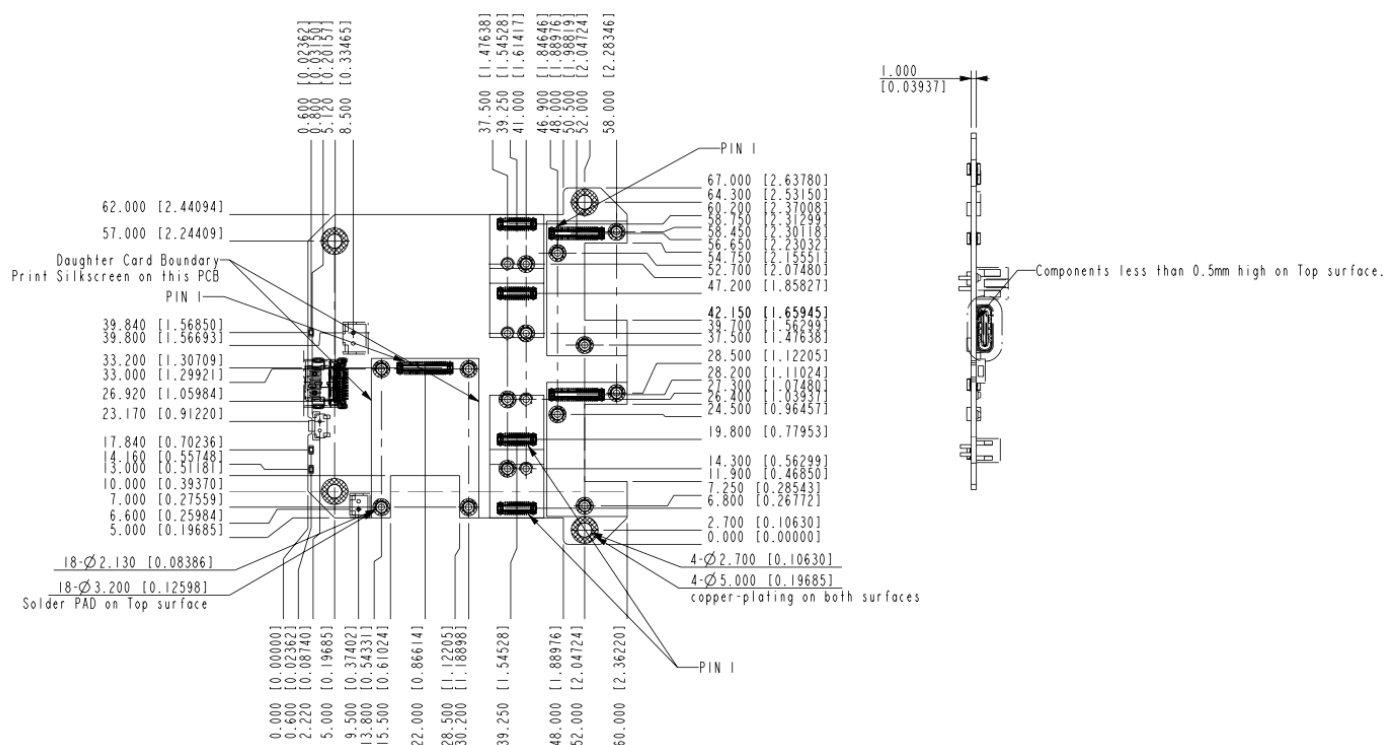
Figure 15: RAK19001 mechanical dimensions
