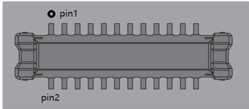
Figure 12: WisBlock 24-pin module connector
