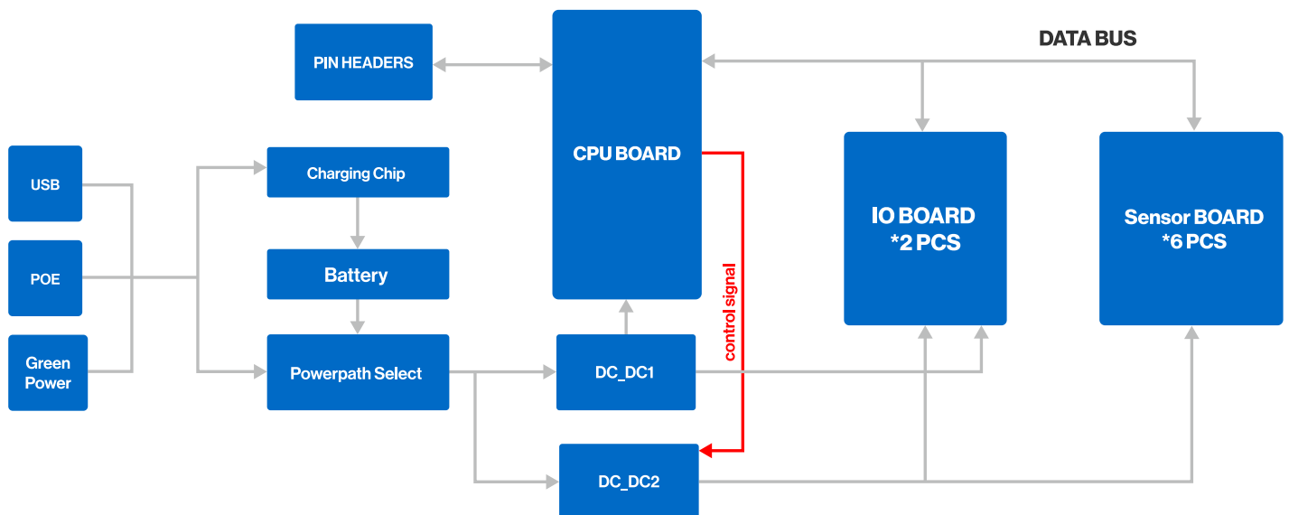
Figure 2: RAK19001 WisBlock Base block diagram
