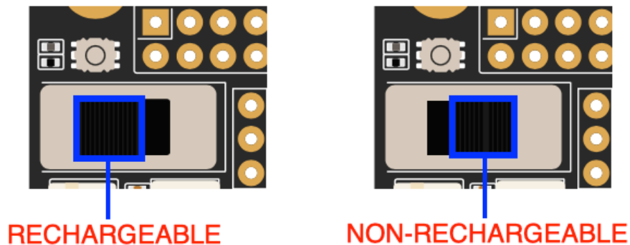
Figure 9: Battery selector switch
