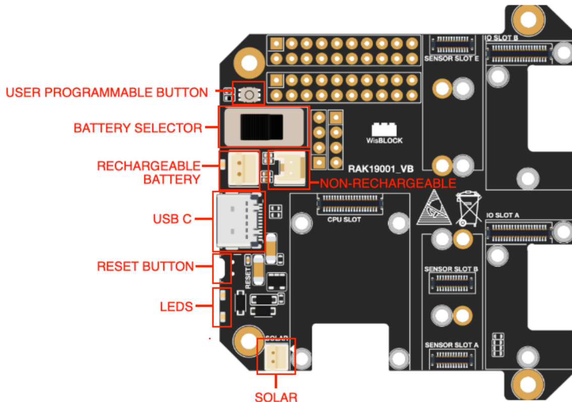
Figure 3: RAK19001 part labels
