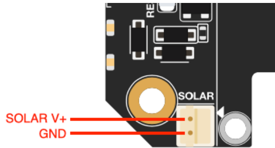
Figure 10: Solar panel connector V+ and GND
