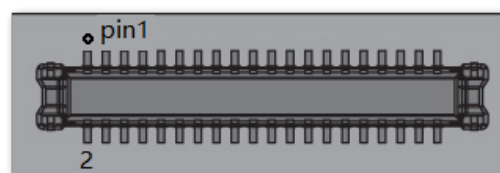
Figure 11: WisBlock Core module 40-pin connector
