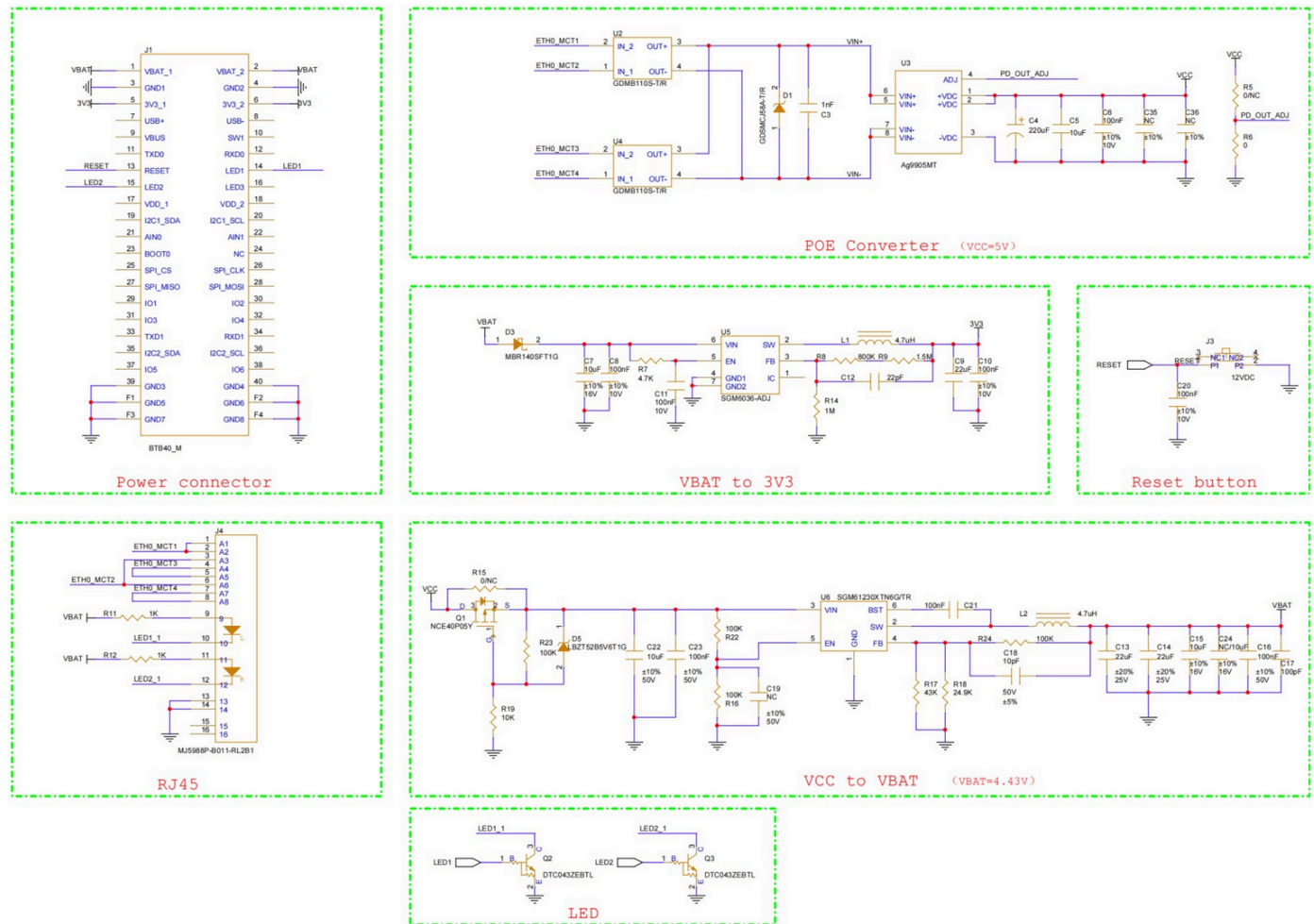
Figure 7: RAK19017 schematic
