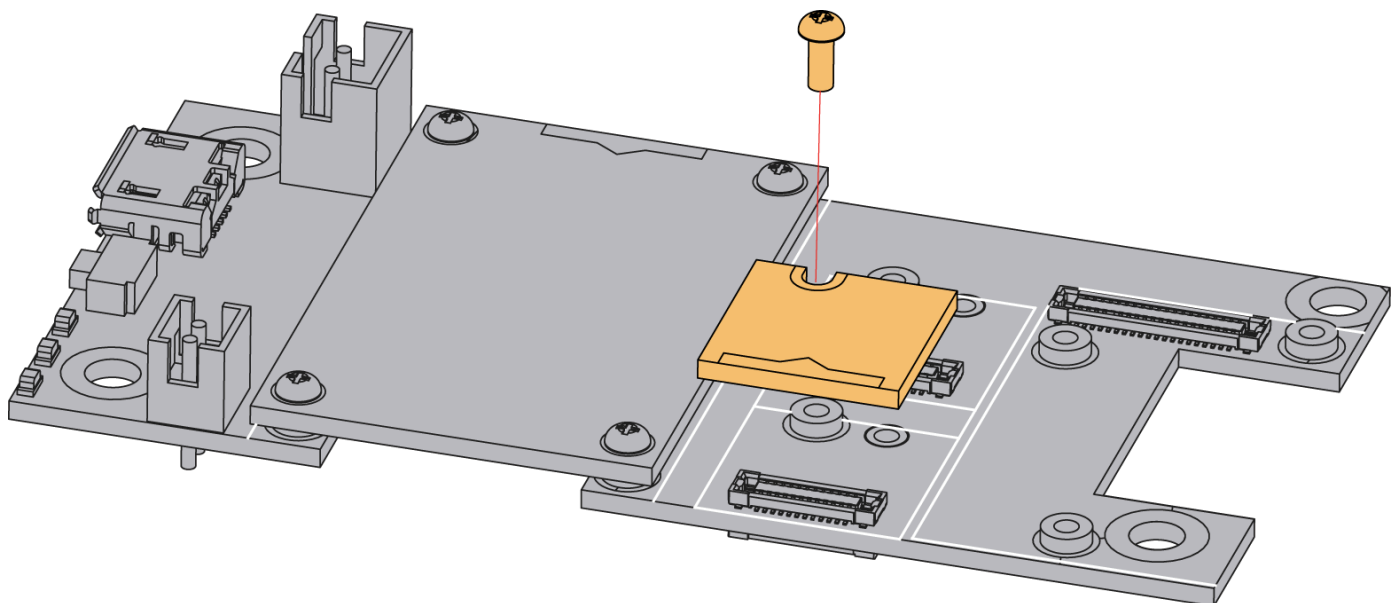
Figure 2: RAK1906 WisBlock Environmental Sensor Mounting
