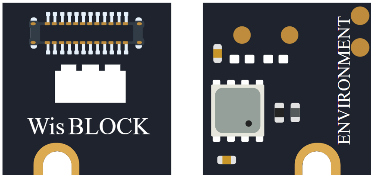
Figure 1: RAK1906 WisBlock Environmental Sensor
