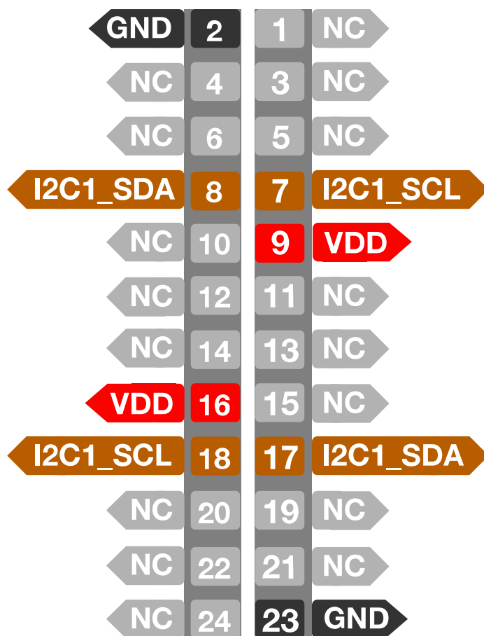
Figure 3: RAK1906 WisBlock Environmental Sensor Pinout
