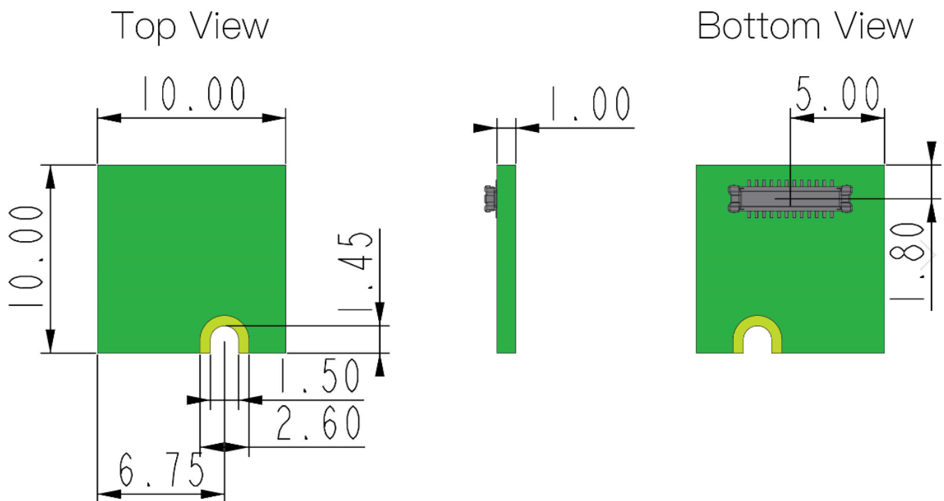
Figure 4: RAK1906 WisBlock Environmental Sensor mechanic dimensions
