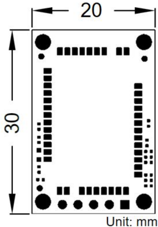
Figure 5: Mechanical Dimensions
