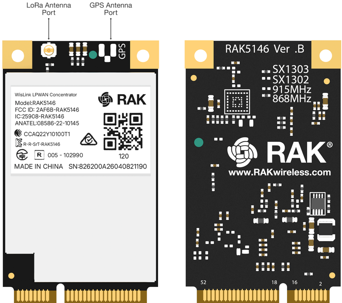
Figure 1: Board Overview
