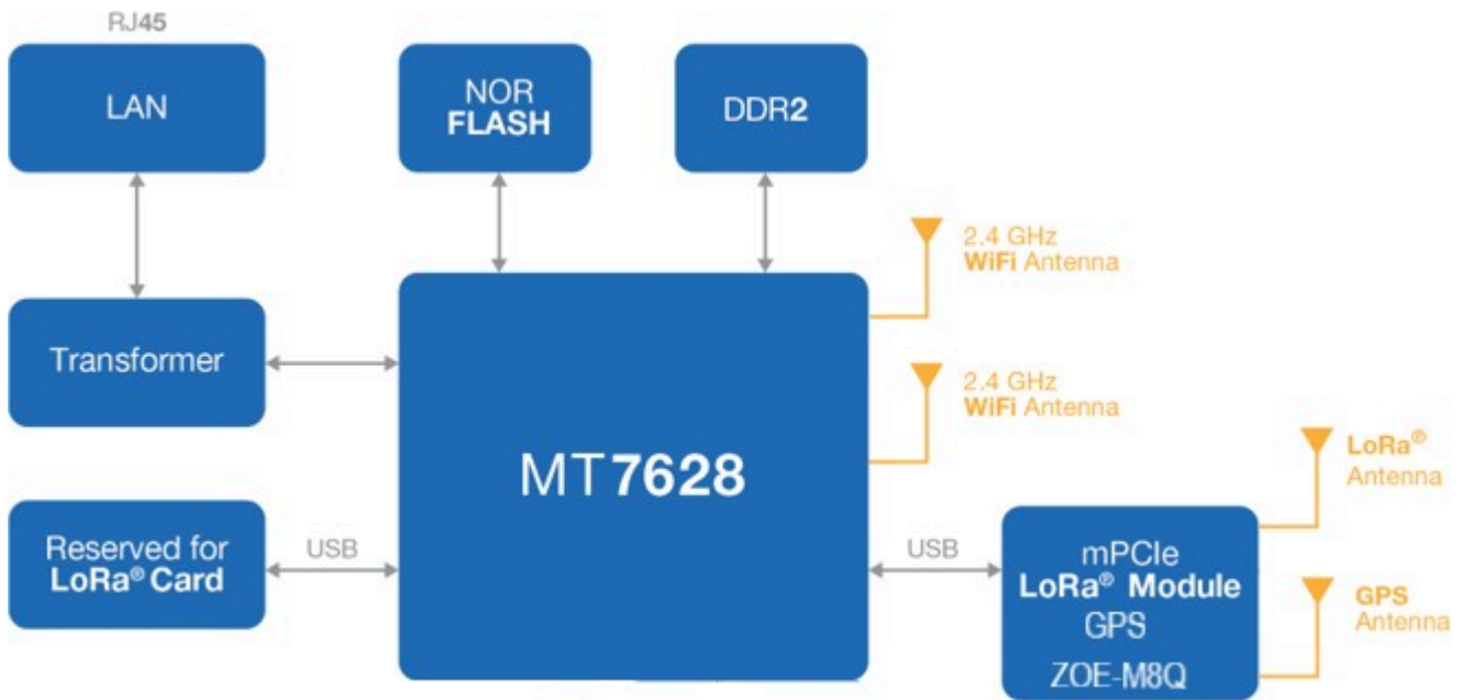
Figure 1: RAK7289V2 Block Diagram
