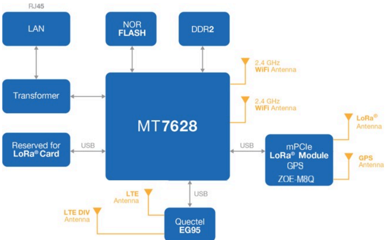
Figure 2: RAK7289CV2 Block Diagram
