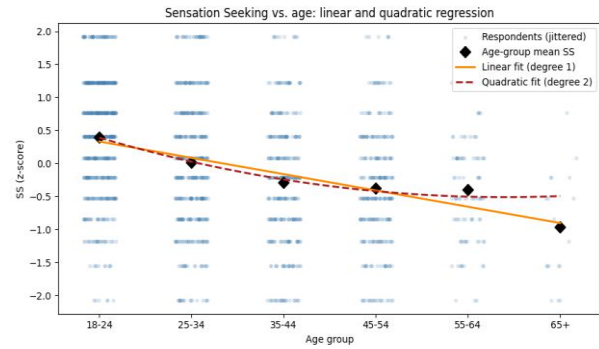
Figure 6: linear vs. quadratic regression.
