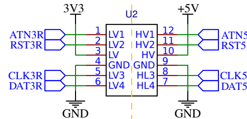
Levelshifter
