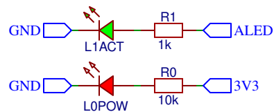
Signalling LEDs
