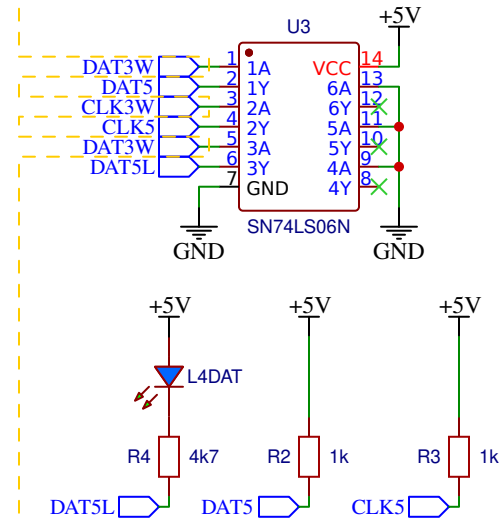
Open collector CLK/DAT
