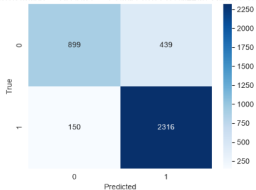
Confusion Matrix — NN base — Feature noise localizzato Rumore 40%
