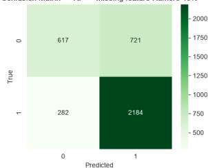
Confusion Matrix — RF — Missing feature Rumore 40%
