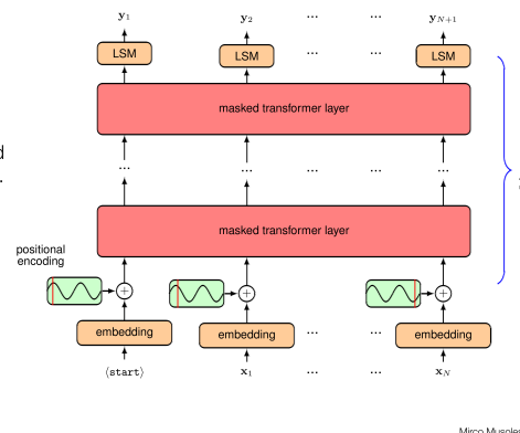
Figure 3: Official Lecture Diagram: Autoregressive GPT Training & Causal Masking.
