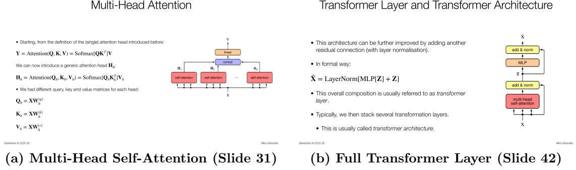
Figure 2: Official Lecture Diagrams: Multi-Head Self-Attention and Full Transformer Architecture.
