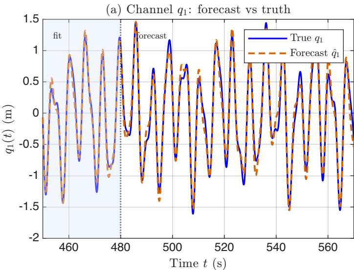
Benchmark 1: Spring–Mass Chain ( N = 4 , observe q_1, q_4 , fixed–free)
