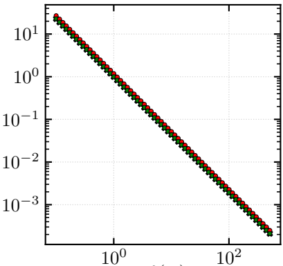
\alpha = 2.386, f(\alpha) \approx 0.57525
