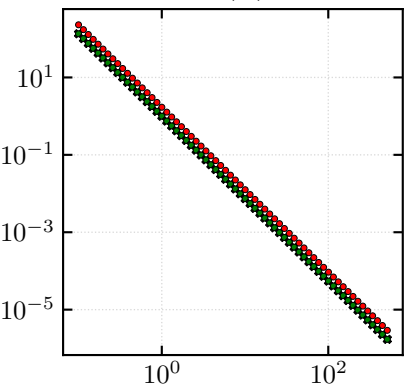
\alpha = 2.129, f(\alpha) \approx 0.62329
