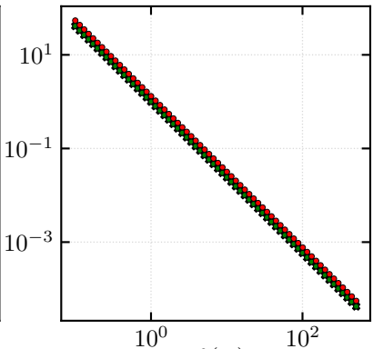
\alpha = 2.643, f(\alpha) \approx 0.48492
