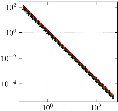
\alpha = 2.9, f(\alpha) \approx 0.29096
