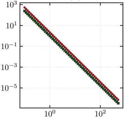
\alpha = 2.386, f(\alpha) \approx 0.57525
