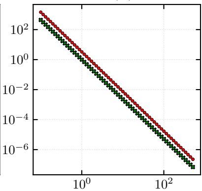
\alpha = 2.643, f(\alpha) \approx 0.48492
