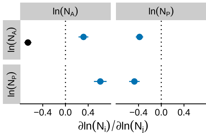
Ecological feedback (A)
