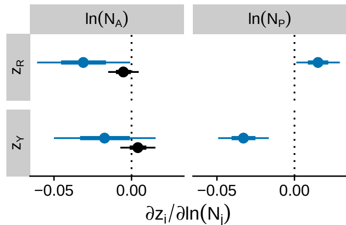
Eco-to-evo effect (C)
