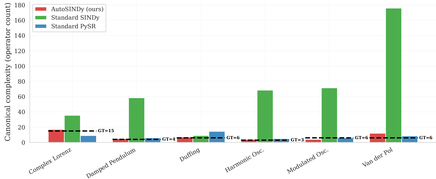
Model Complexity — Median across all noise levels & trials — dashed line = ground-truth equation complexity
