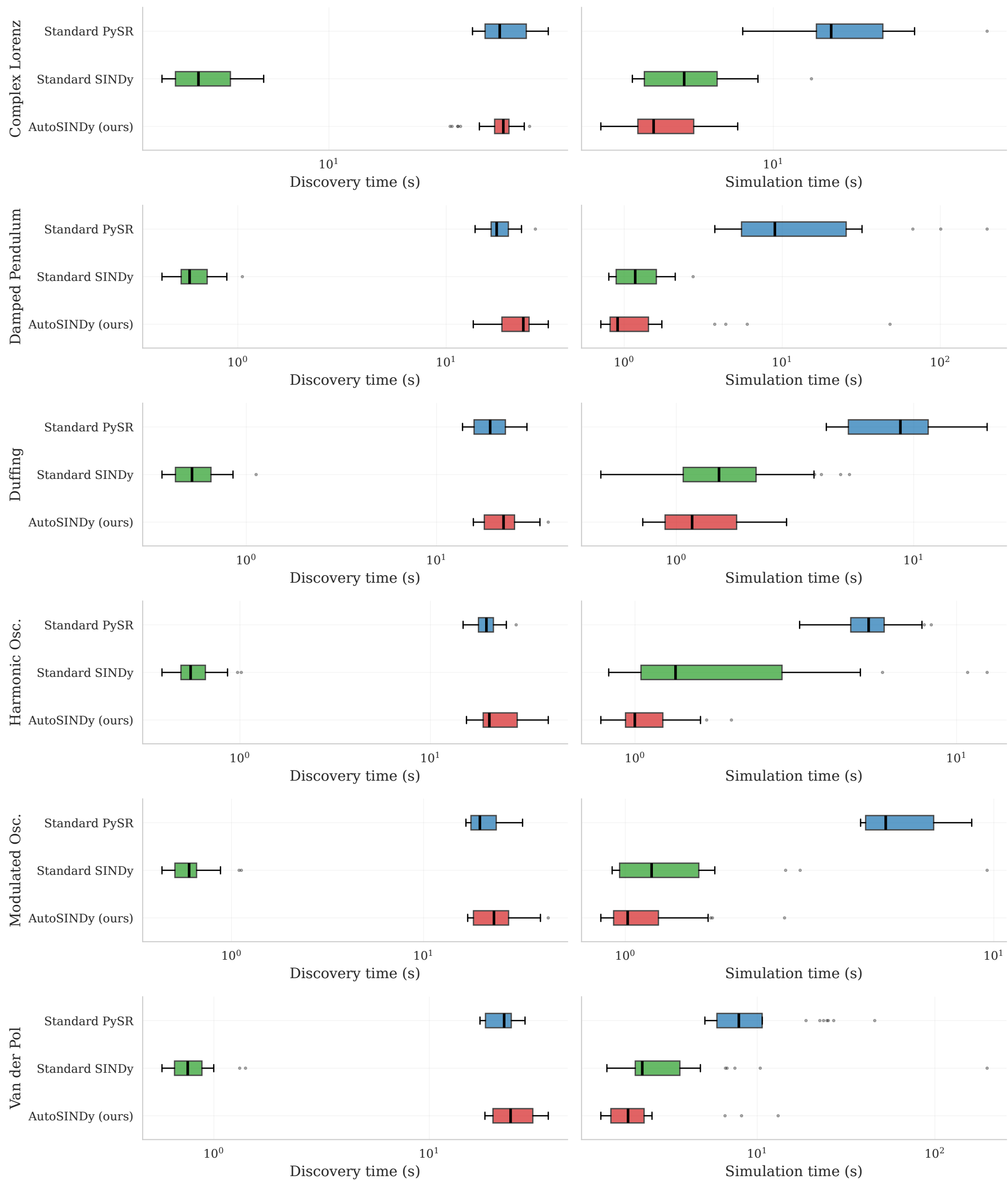
Computation Time — Discovery (left) and Simulation (right)
