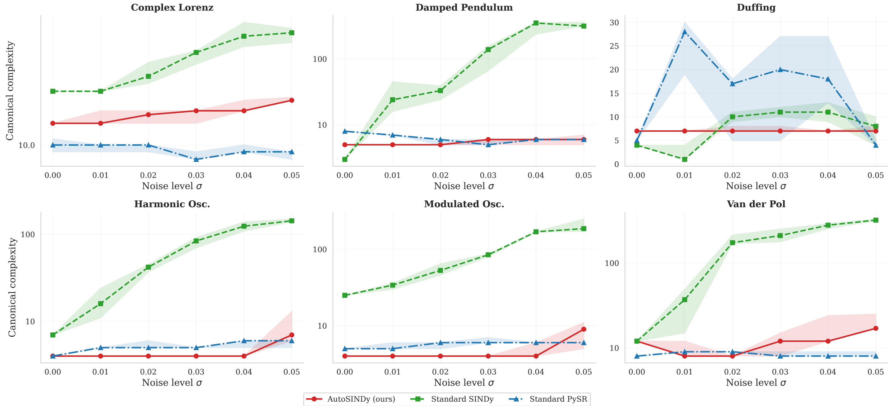
Model Complexity Growth with Noise (median + IQR across trials; log scale when range > 1 decade)
