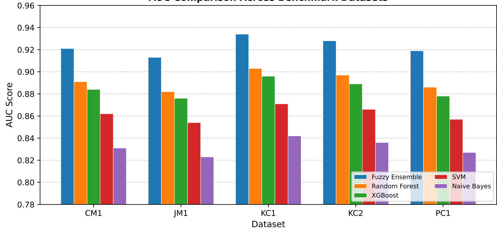
AUC Comparison Across Benchmark Datasets
