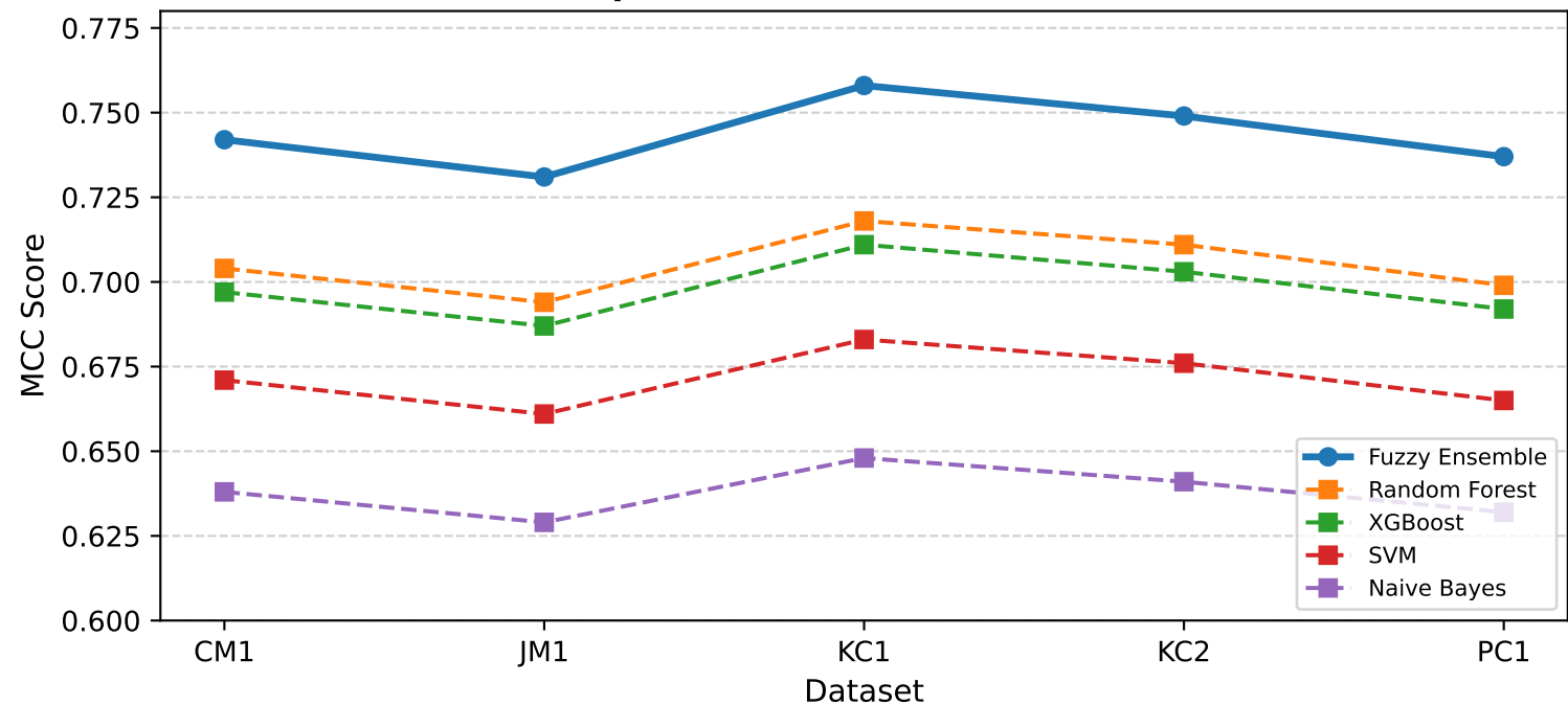
MCC Comparison Across Benchmark Datasets
