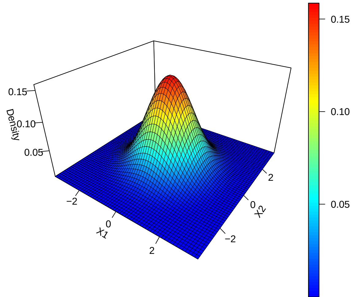
(a) Standard Multivariate Normal
