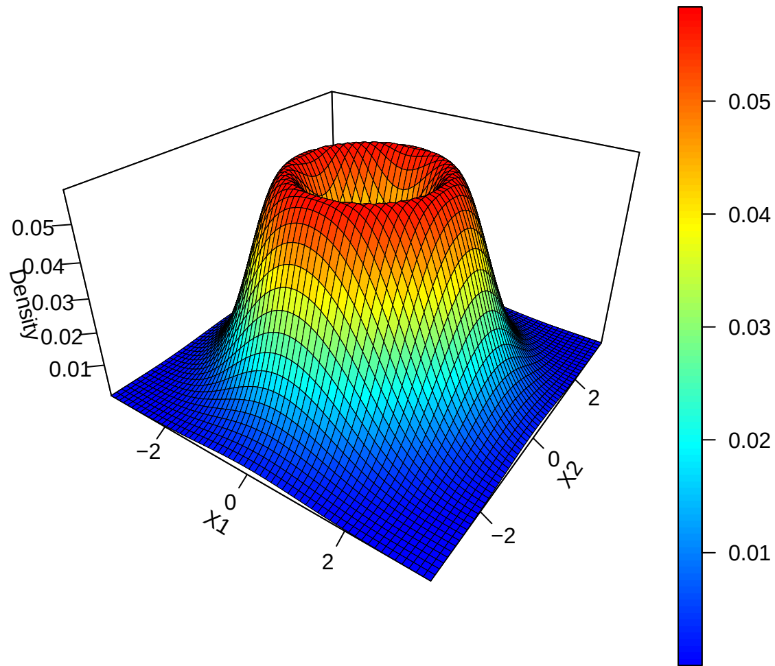
(b) Mahalanobis-Weighted MVN
