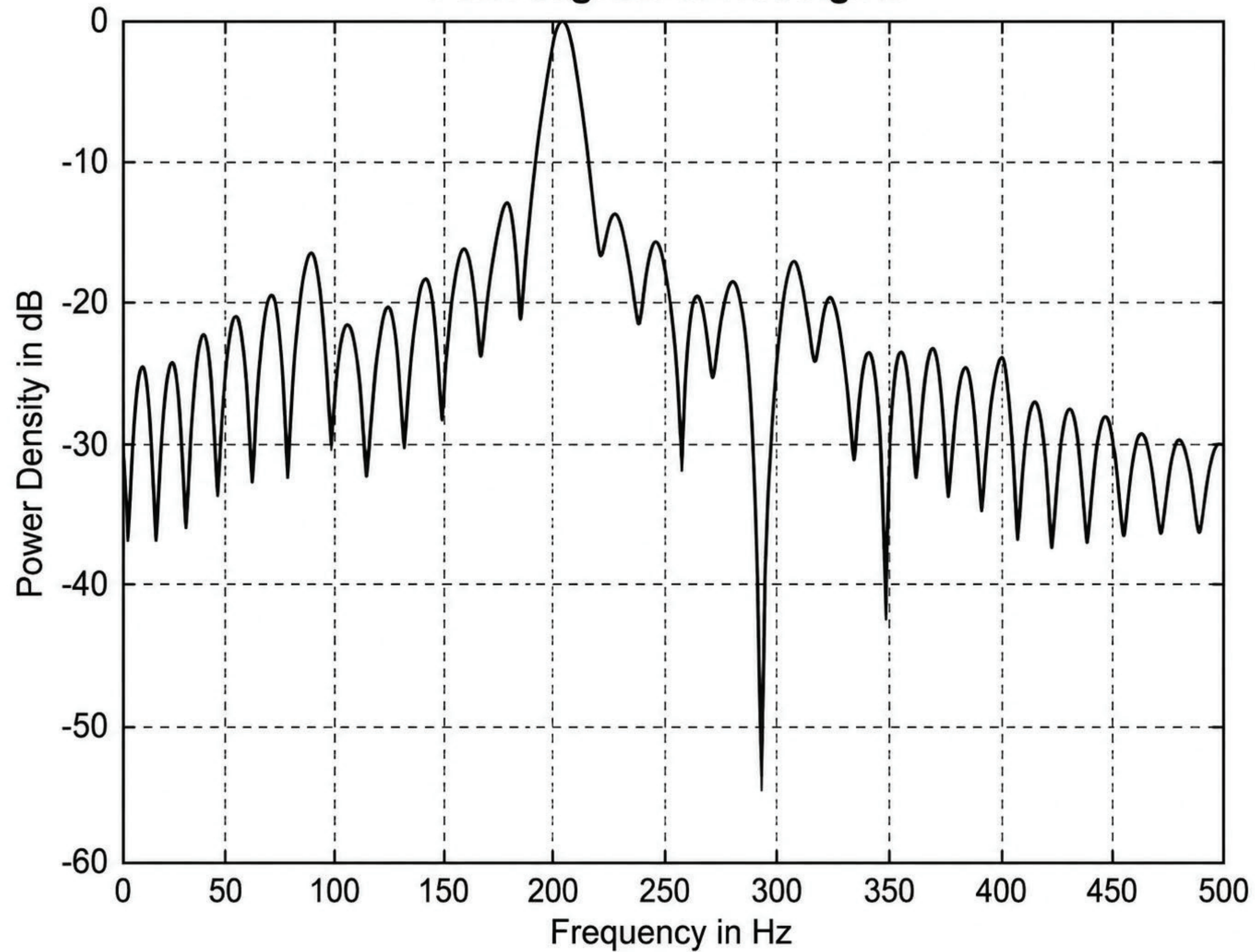
Periodogram of test signal
