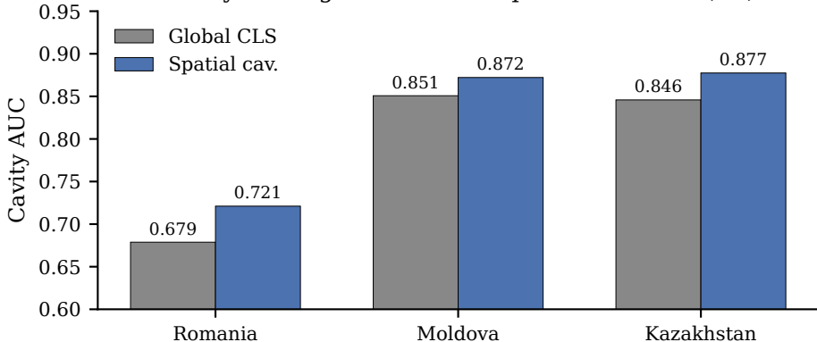
Cavity head: global CLS vs. spatial attention (A2)
