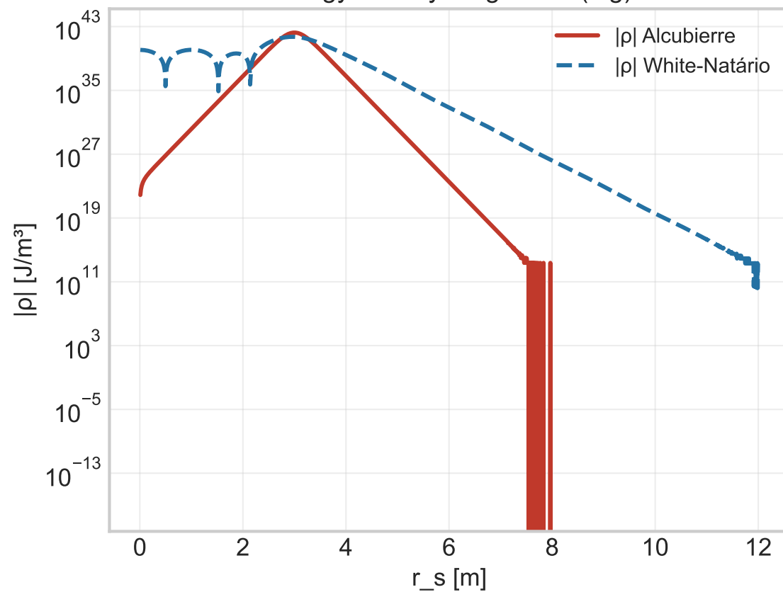
Energy density magnitude (log)
