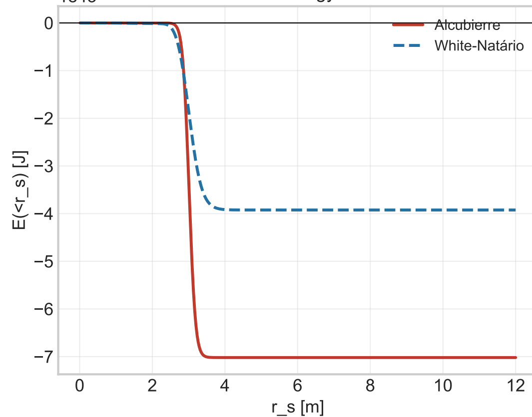
Cumulative energy enclosed
