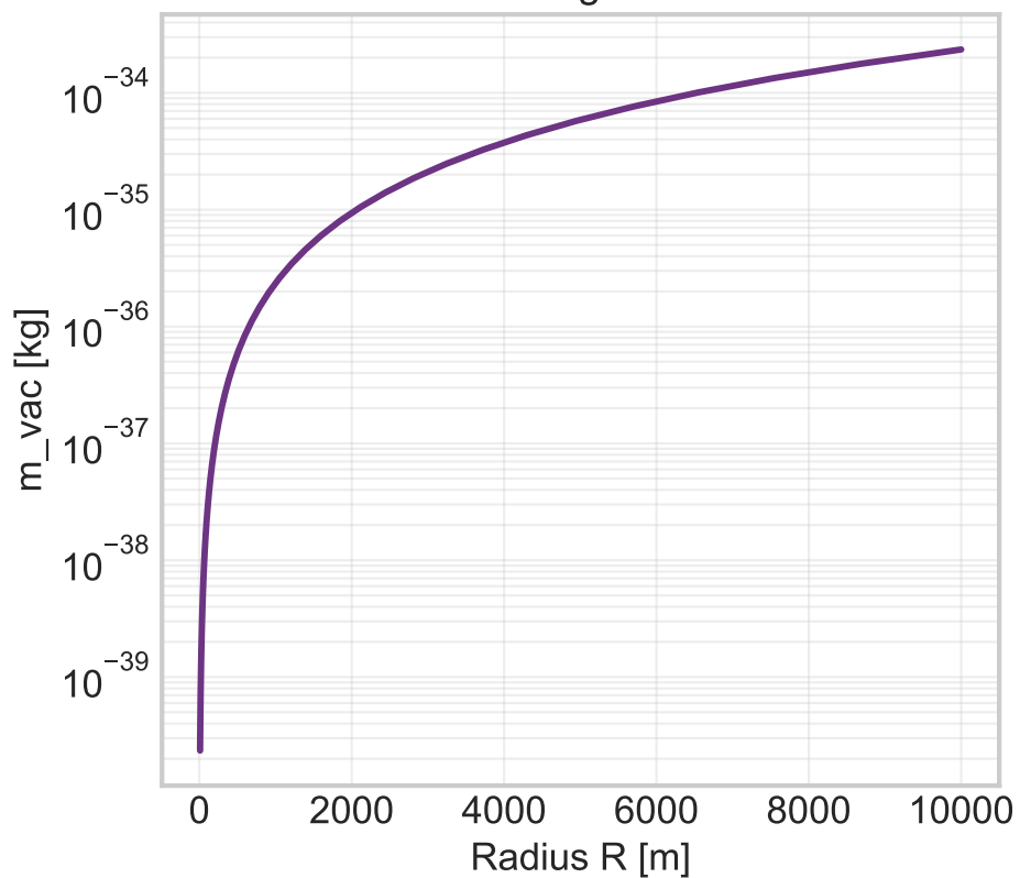
Effective negative mass
