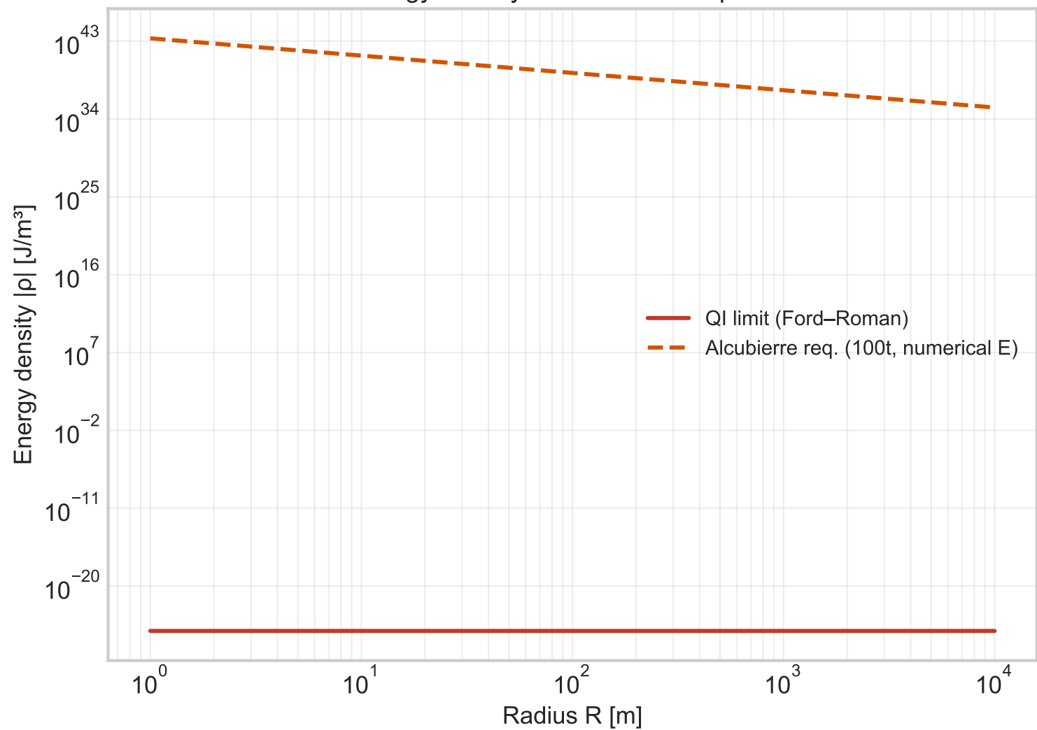
QI energy density vs Alcubierre requirement
