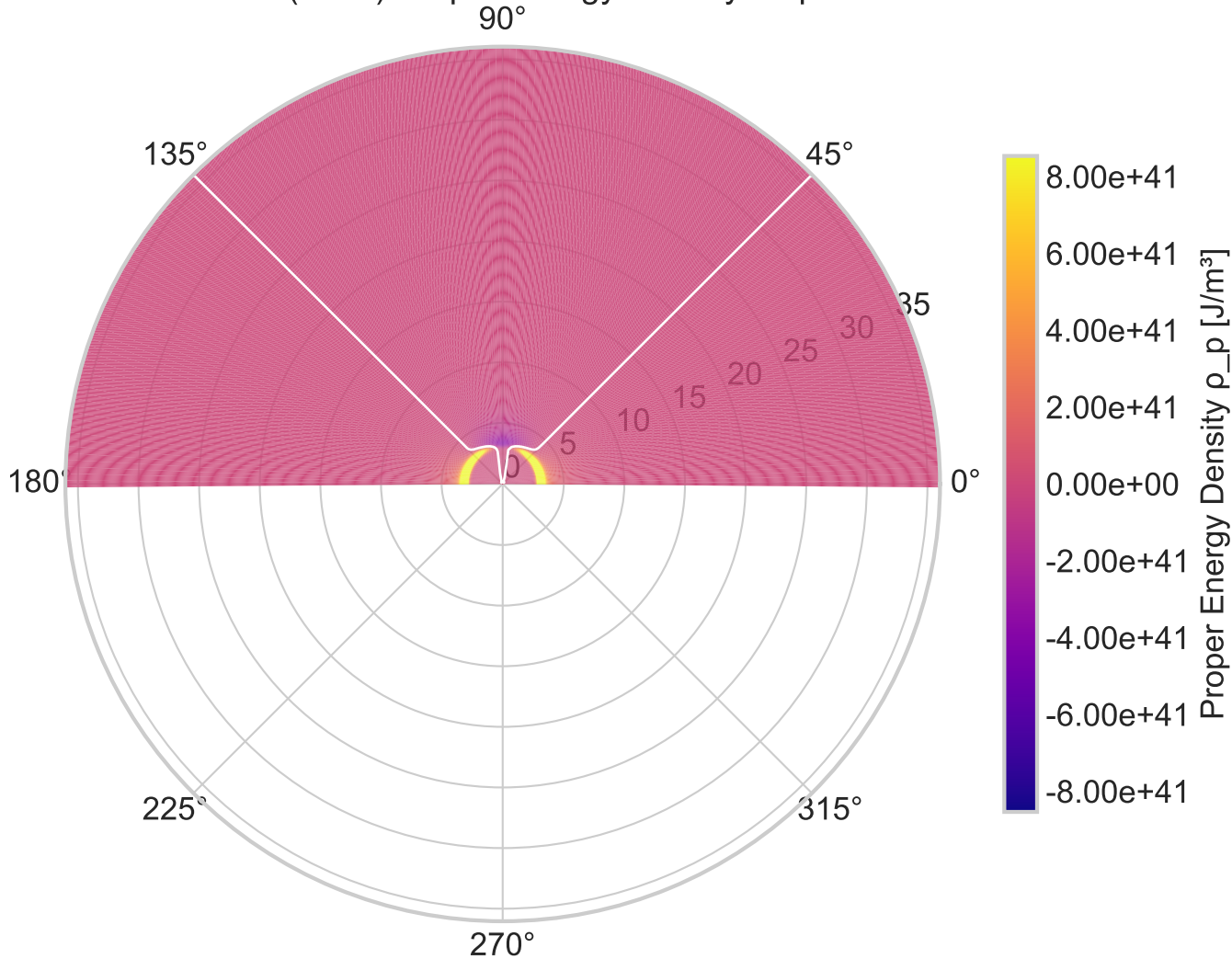
Rodal (2025) Proper Energy Density Map
