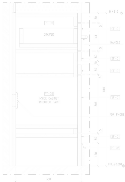
DETAIL-1-1 SCALE 1:1/6
