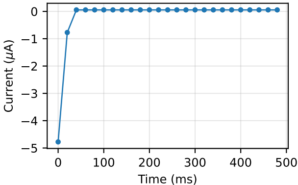
CA transient, 0 to +200 mV step
