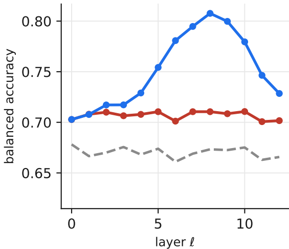
Sim-A (independent layers)
