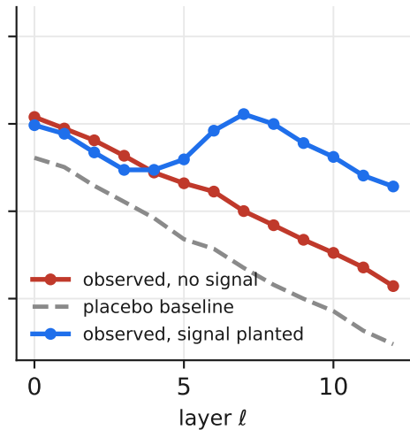
Sim-B (residual stream)
