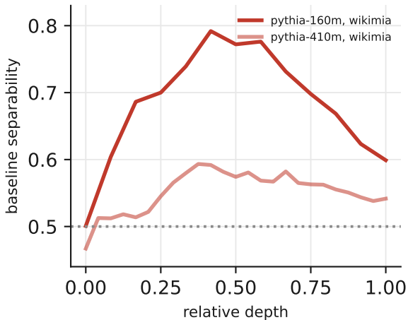
temporal split (WikiMIA)
