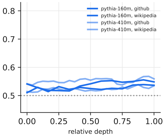
matched split (Pile train vs. val)
