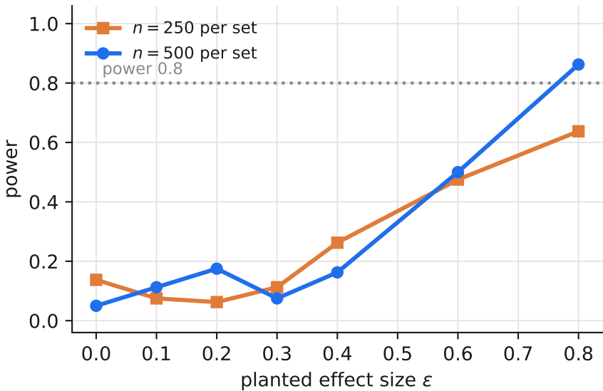
Power of the depth contrast
