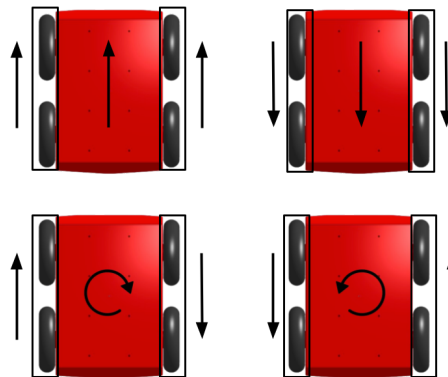
Figure 9.1: Differential Drive Movement Diagram (From Robot Proving Grounds)
