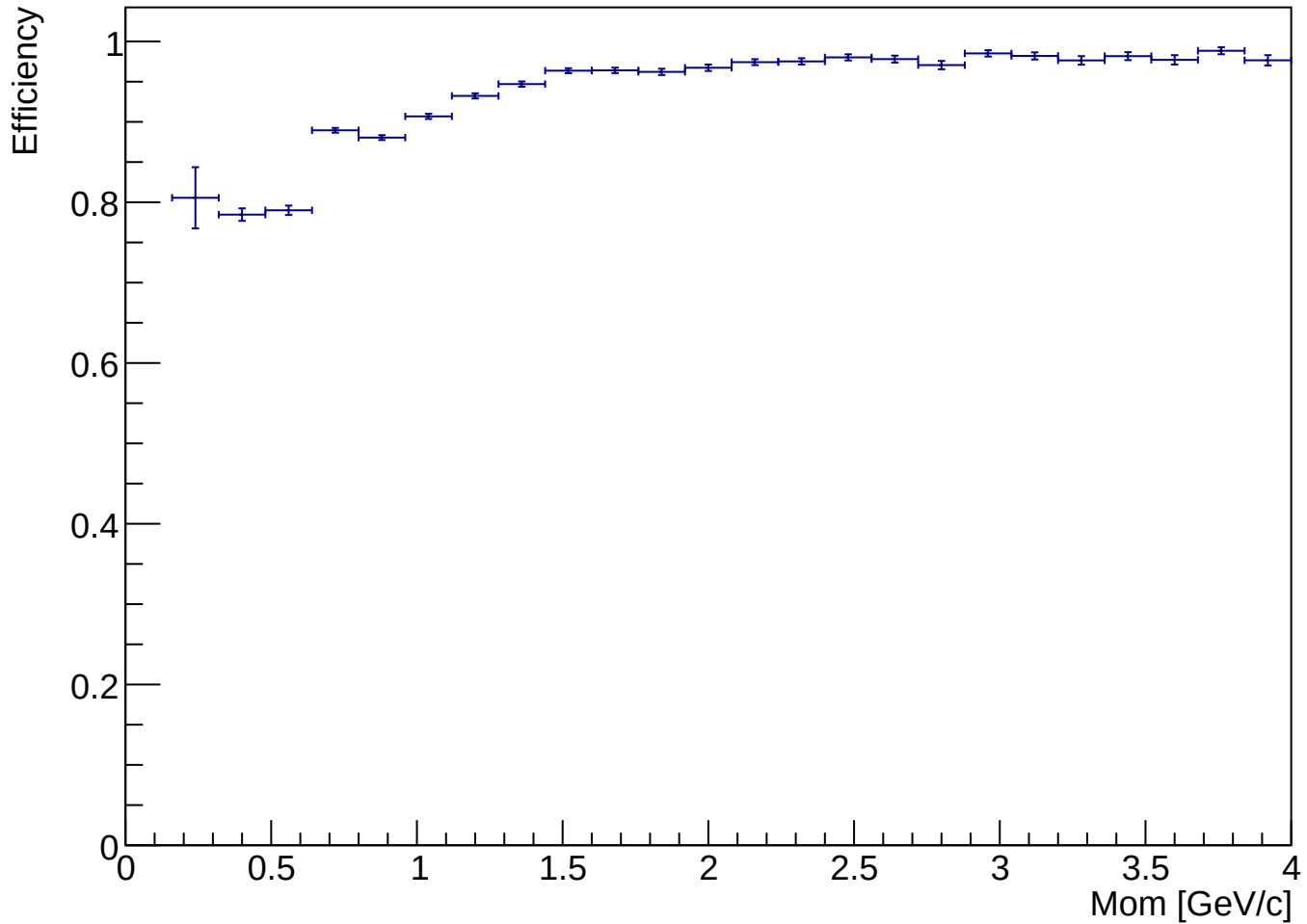
Muon ID Efficiency (id/found)
