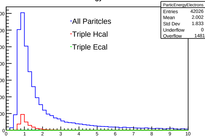
ParticEnergyElectrons
