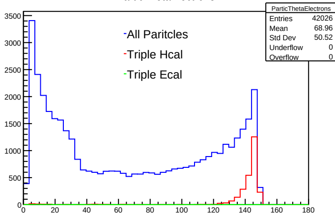
ParticThetaElectrons
