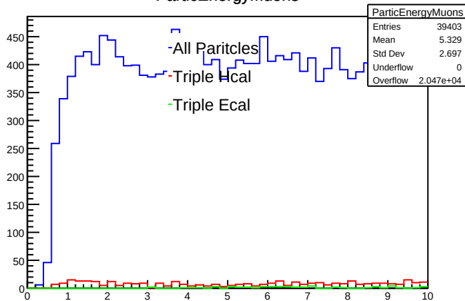
ParticEnergyMuons
