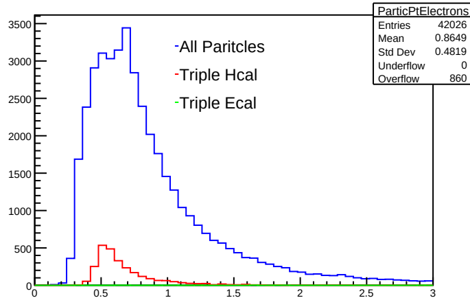
ParticPtElectrons
