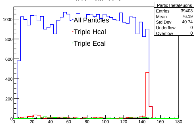
ParticThetaMuons
