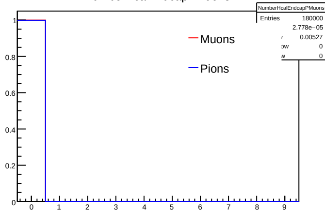
NumberHcalEndcapPMuons
