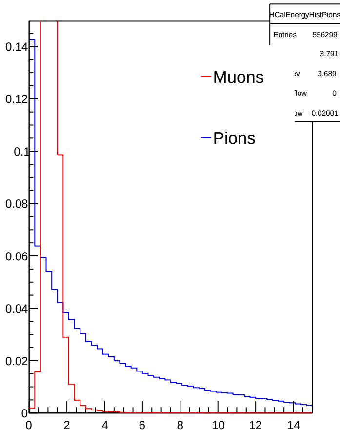
HCalEnergyHistPions
