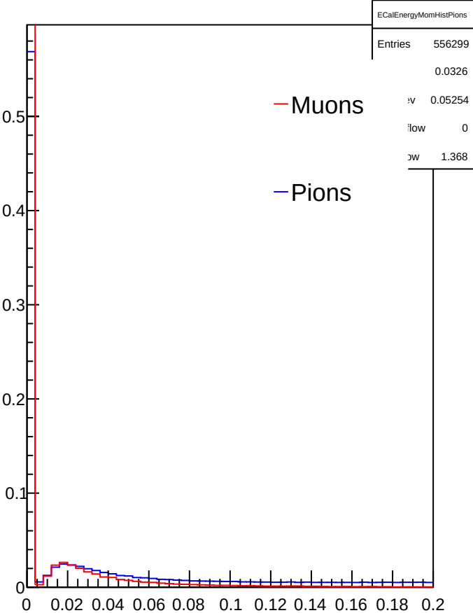
ECalEnergyMomHistPions
