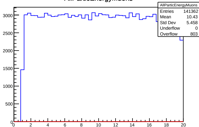
AllParticEnergyMuons
