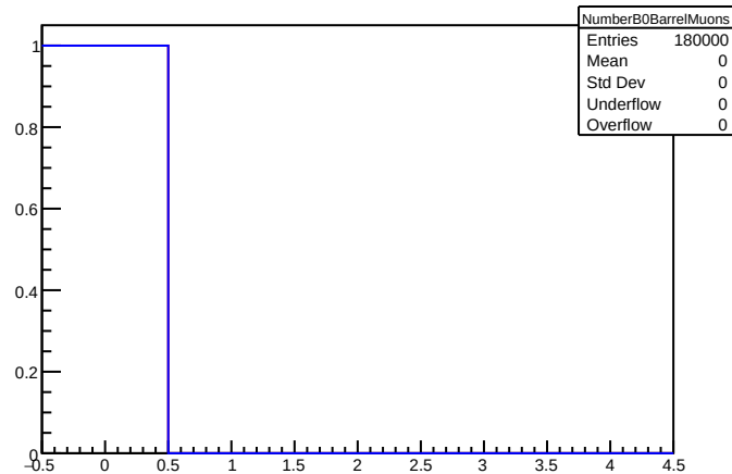
NumberB0BarrelMuons
