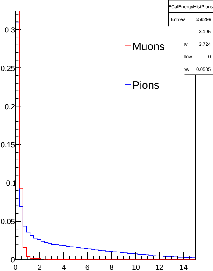
ECalEnergyHistPions
