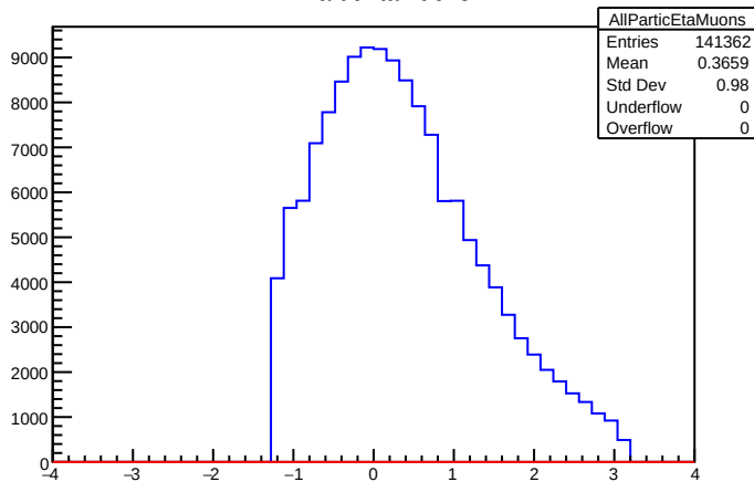
AllParticEtaMuons
