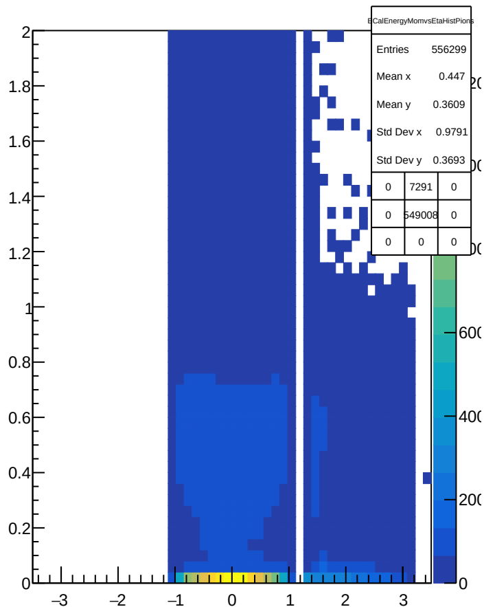
ECalEnergyMomvsEtaistPions
