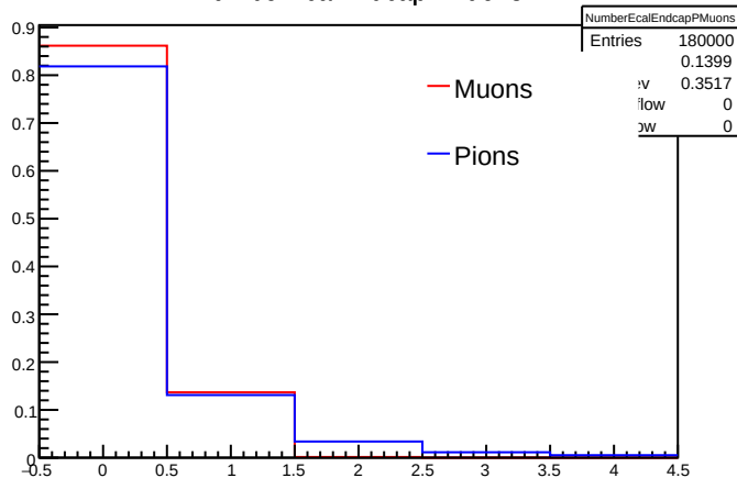
NumberEcalEndcapPMuons
