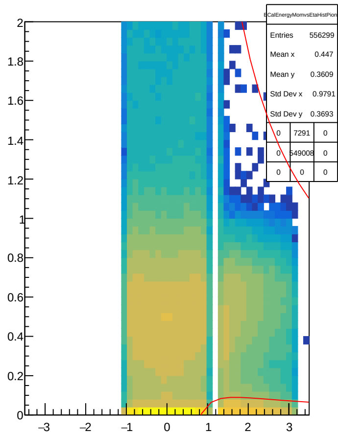
ECalEnergyMomvsEtaHistPions
