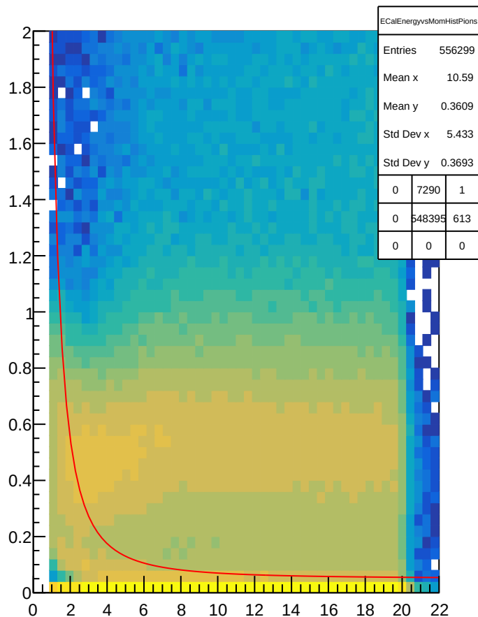
ECalEnergyvsMomHistPions
