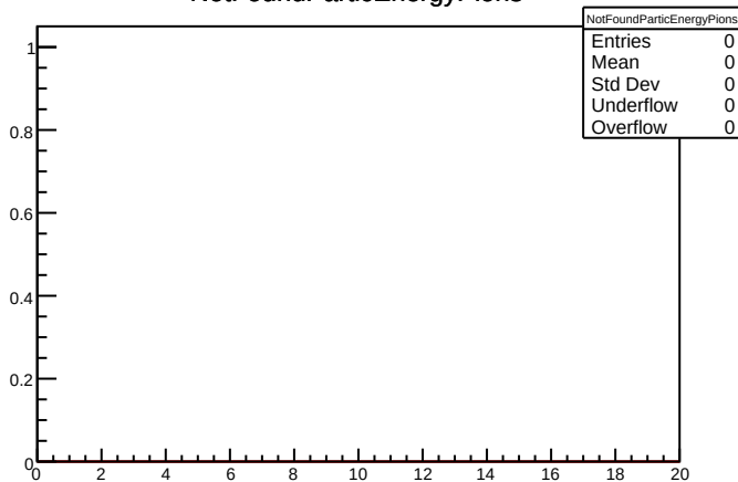
NotFoundParticEnergyPions
