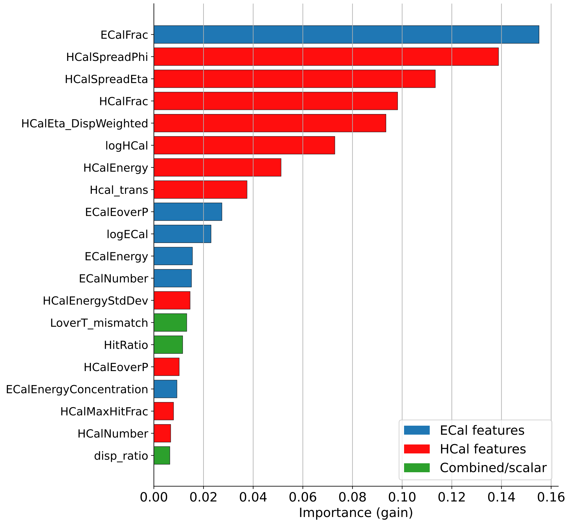
Top 20 Features
