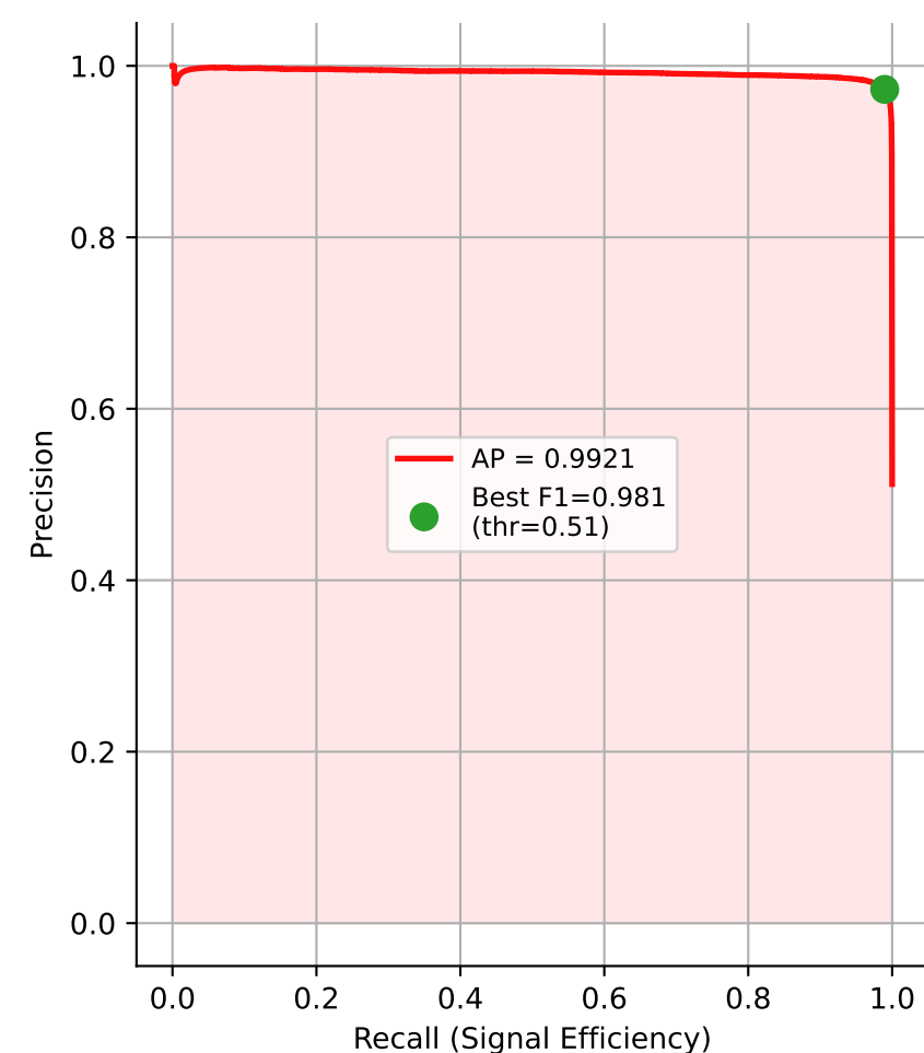
Precision-Recall Curve
