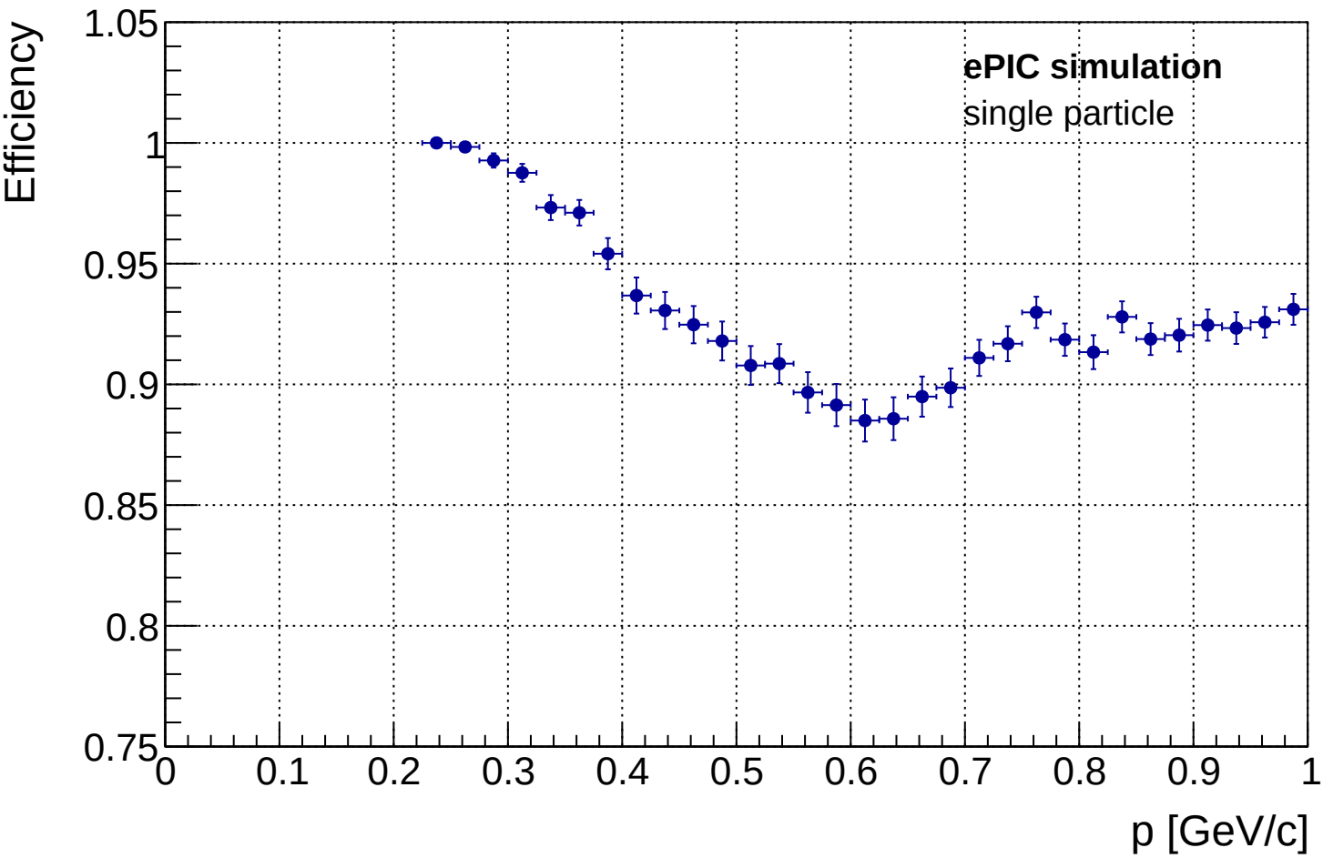
Muon Efficiency vs p (with ToF)
