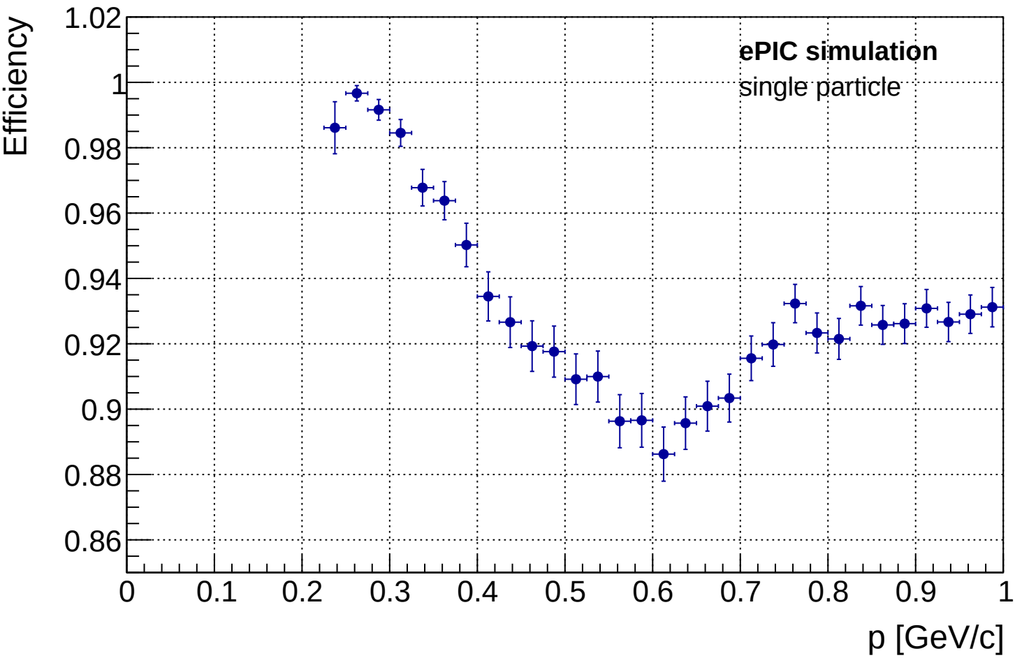
Muon Efficiency vs p (Low p)
