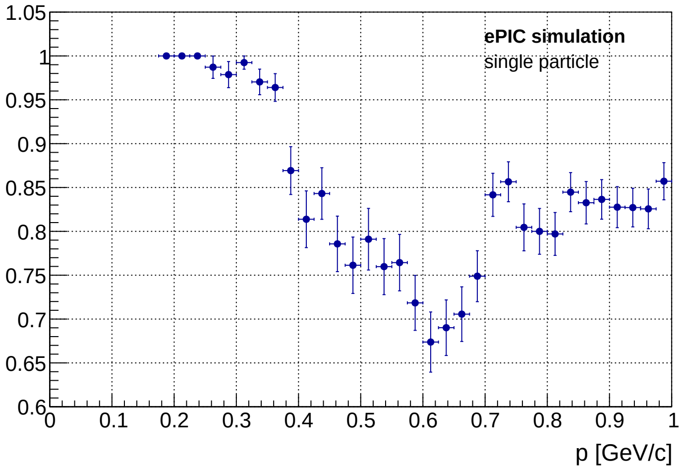
Pion Rejection vs p (Low p)
