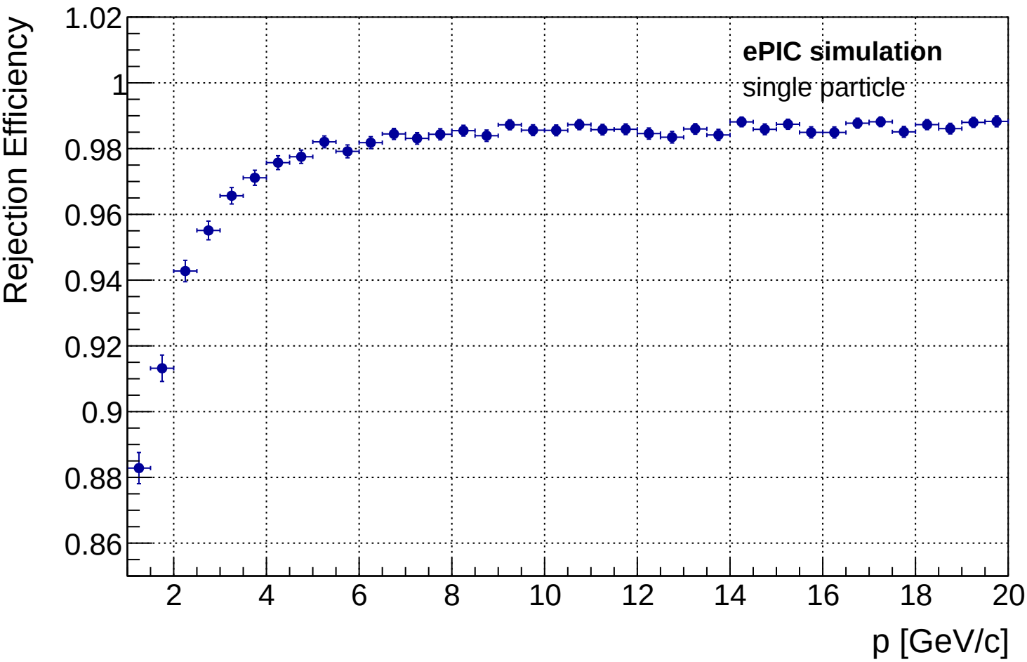
Pion Rejection vs p (High p)
