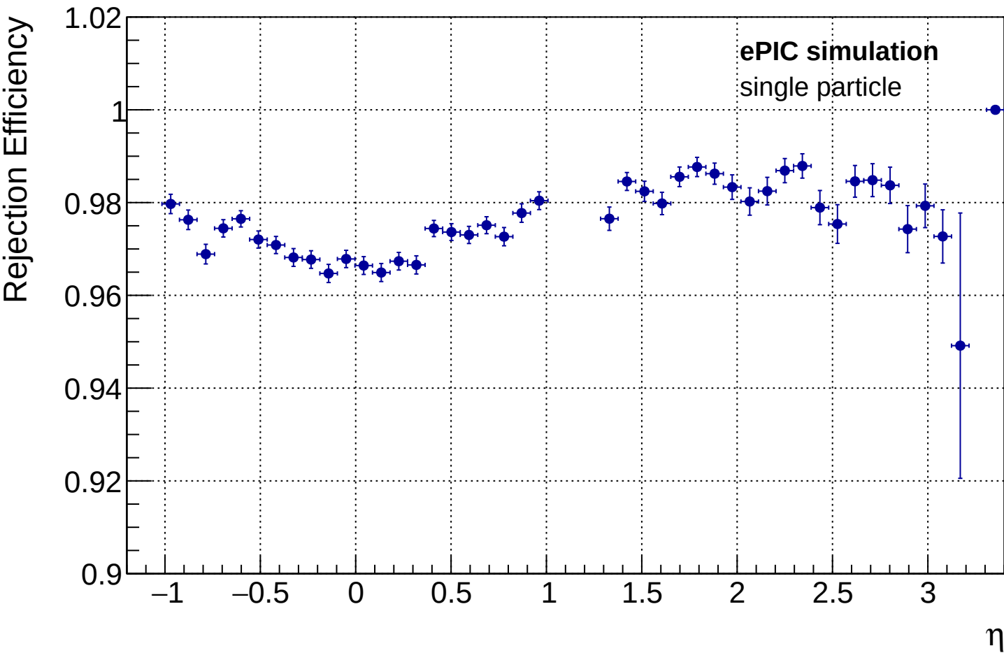
Pion Rejection vs \eta
