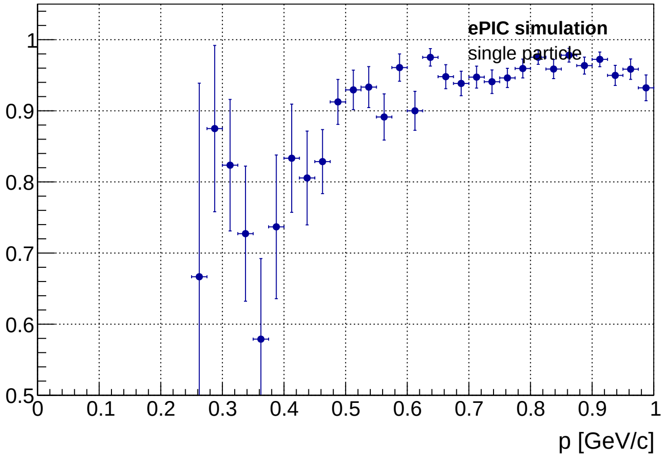
Muon Efficiency vs p (no ToF)
