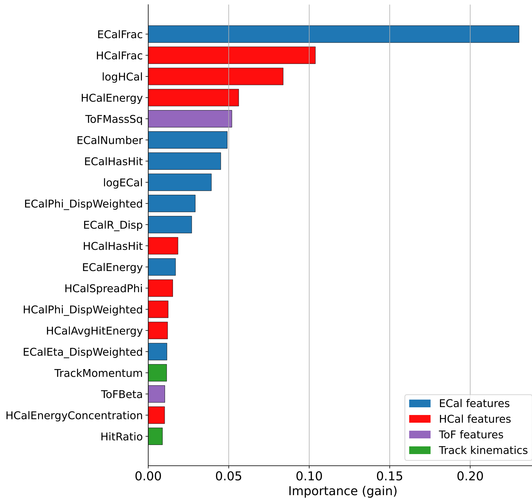
Top 20 Features
