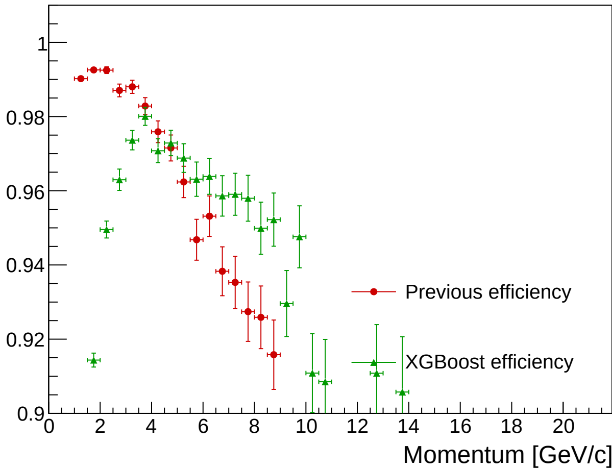
Muon Candidate Efficiency vs p
