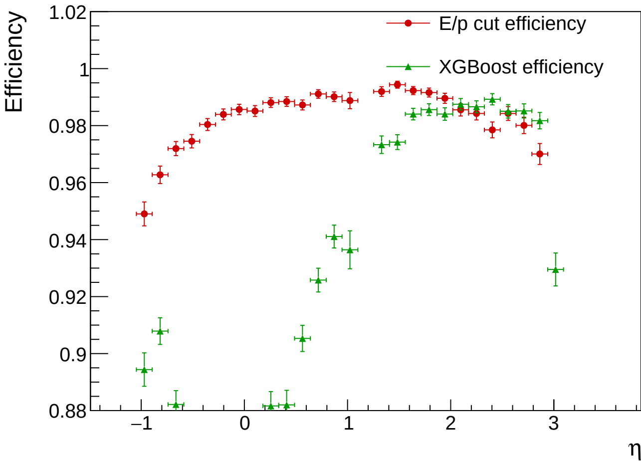
Muon Candidate Efficiency vs \eta
