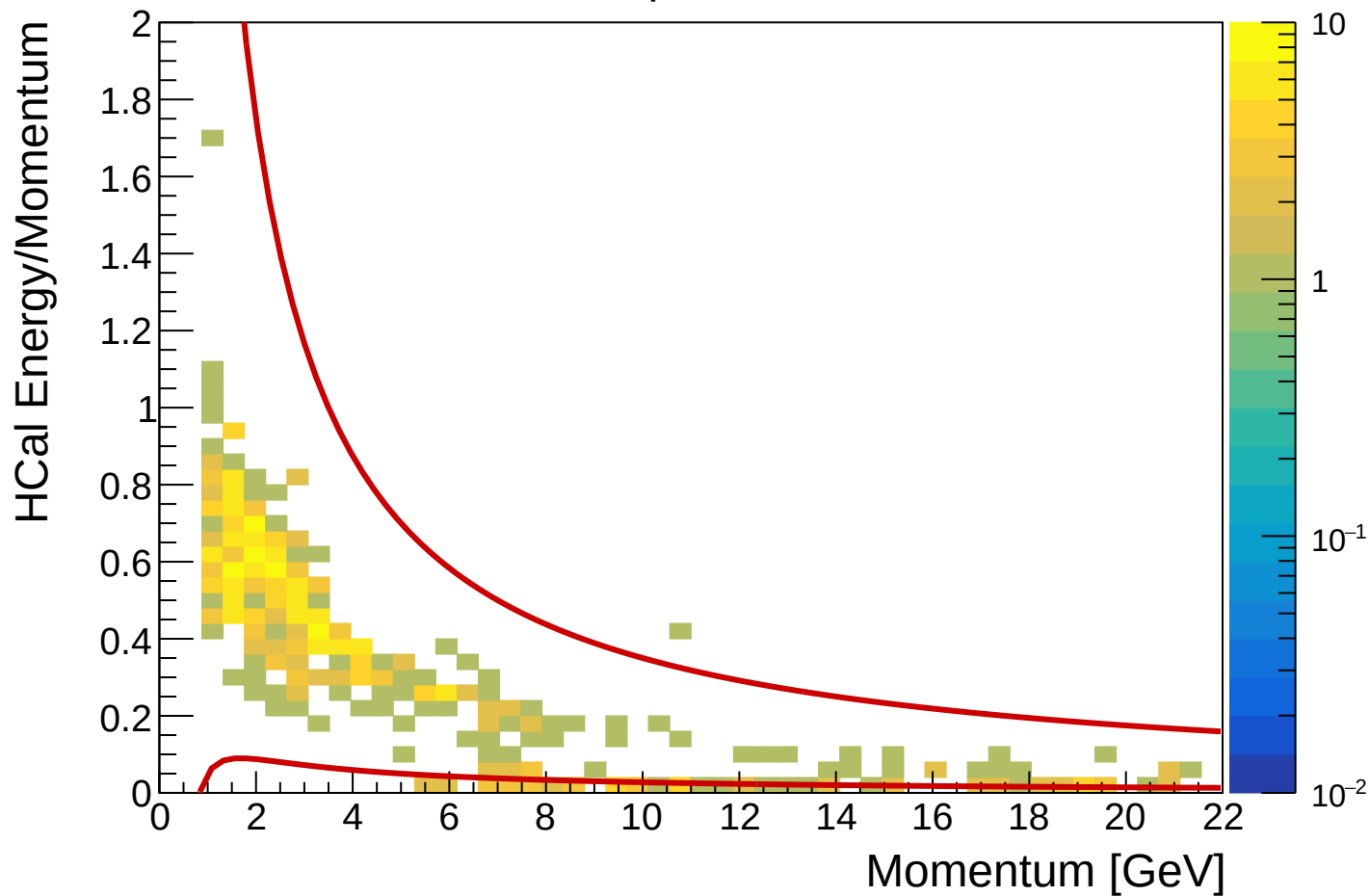
HCal Response to Pions
