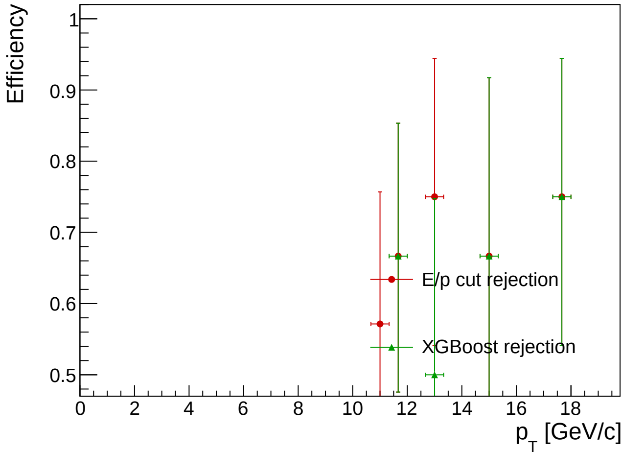
Pion Rejection vs p_T
