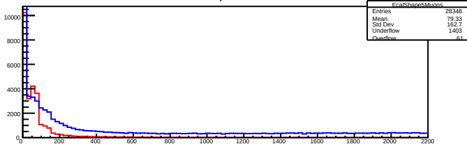
EcalShape5Muons
