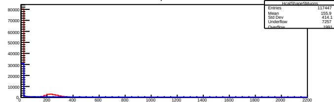
HcalShape5Muons
