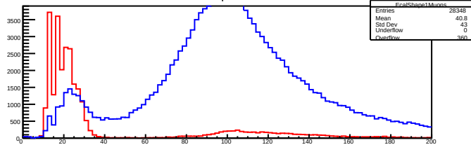
EcalShape1Muons
