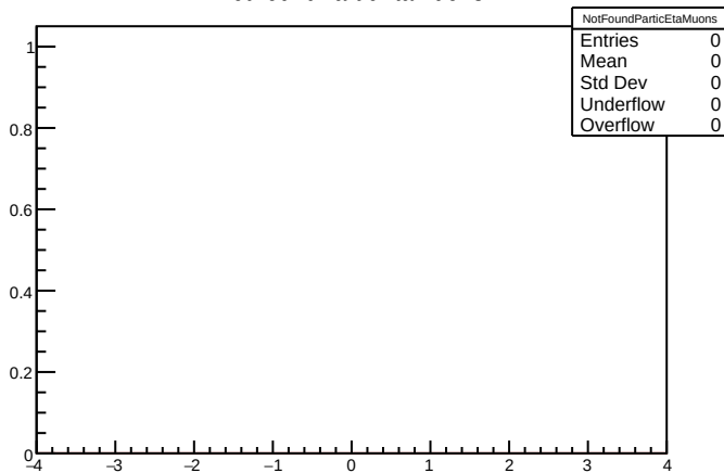
NotFoundParticEtaMuons
