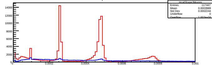
HcalShape3Muons
