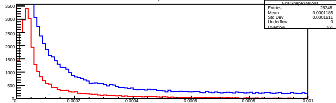
EcalShape3Muons
