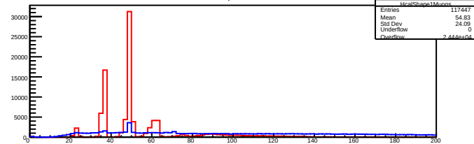
HcalShape1Muons
