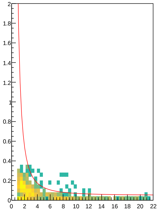
ECalEnergyvsMomHistPions
