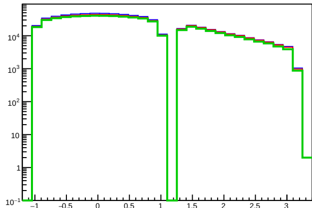
AllParticEtaPions
