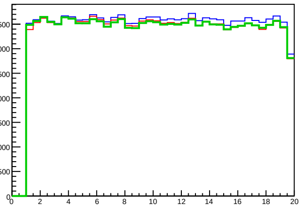
AllParticEnergyMuons
