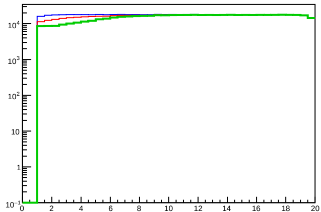
AllParticEnergyPions
