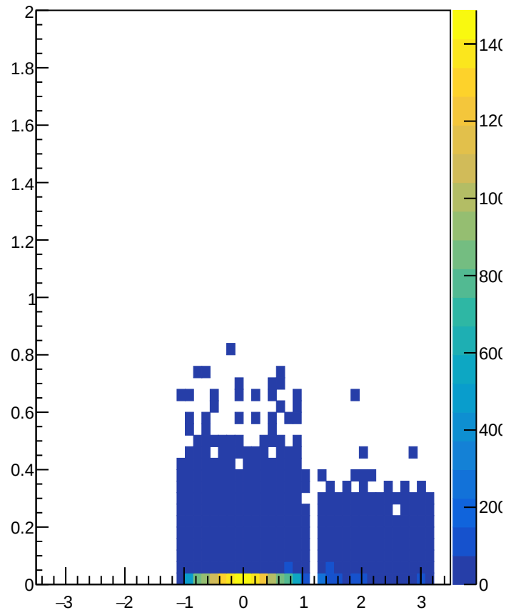
ECalEnergyMomvsEtaistPions
