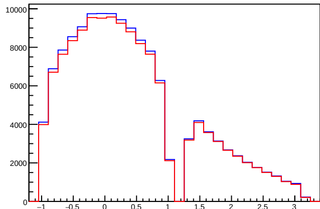
AllParticEtaMuons
