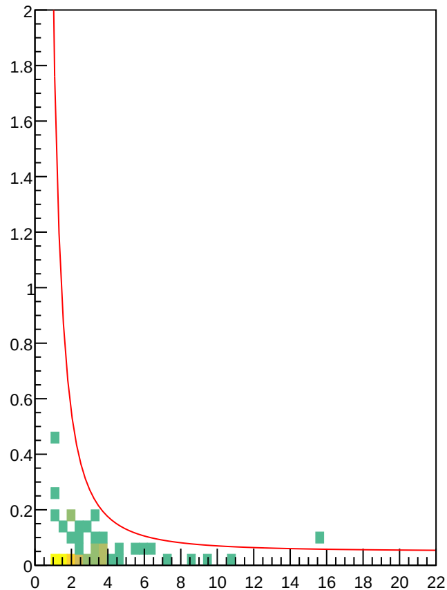
ECalEnergyvsMomHistPions
