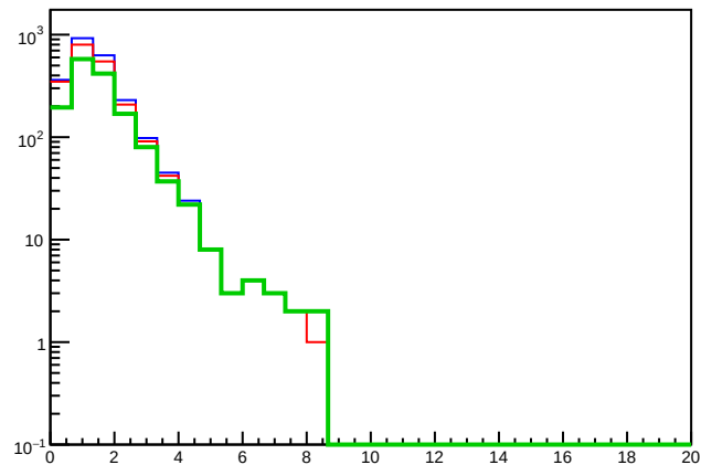
AllParticPtPions
