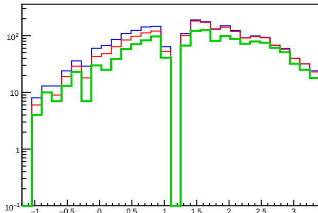
AllParticEtaPions
