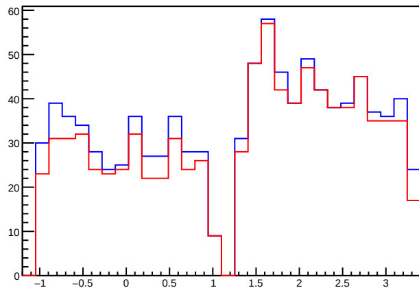
AllParticEtaMuons
