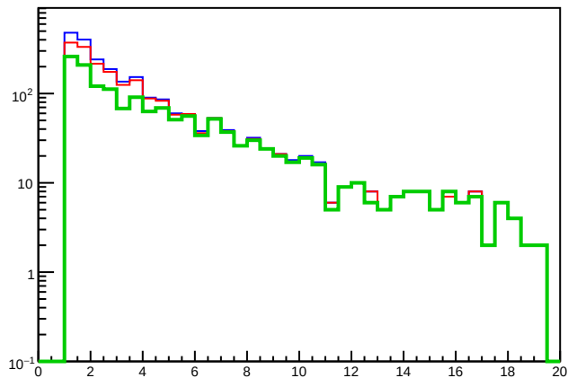
AllParticEnergyPions
