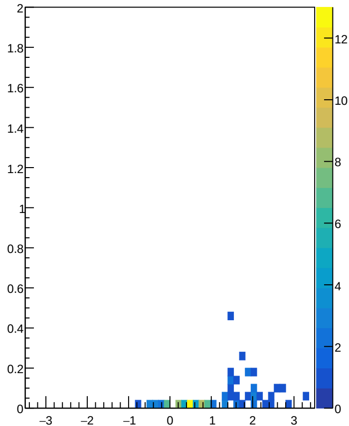
ECalEnergyMomvsEtaistPions
