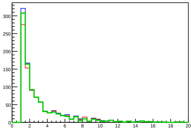
AllParticEnergyMuons
