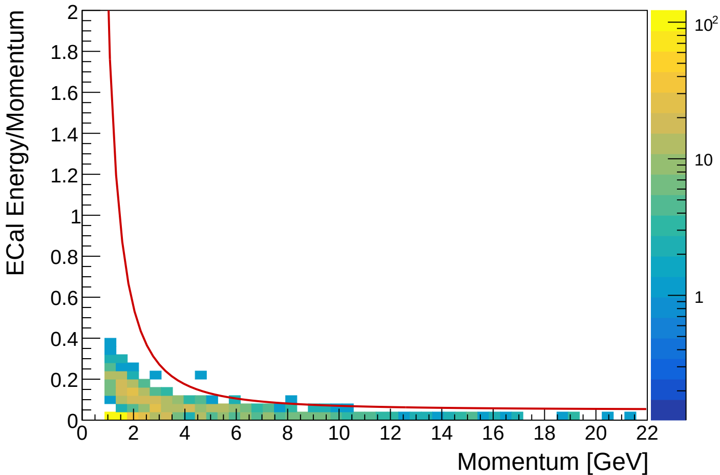
ECal Response to Muons
