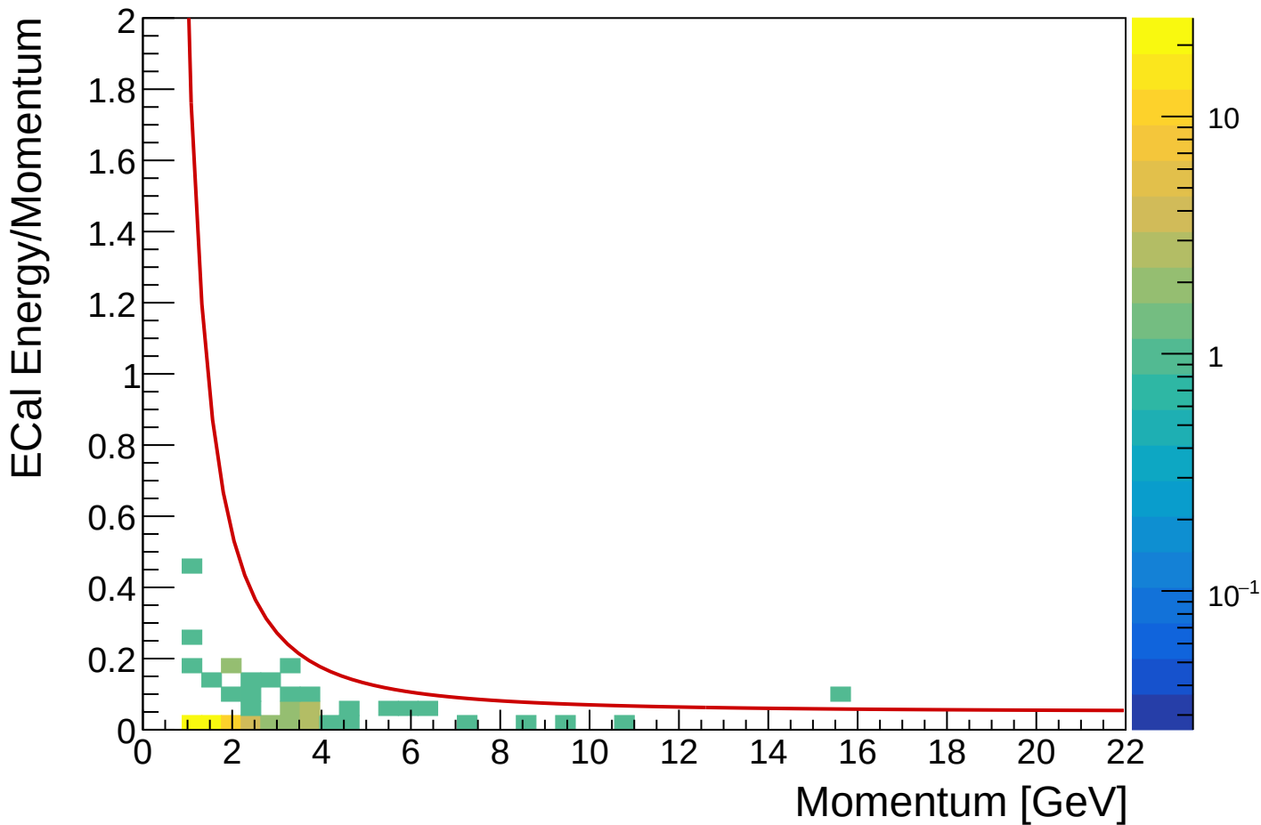
ECal Response to Pions
